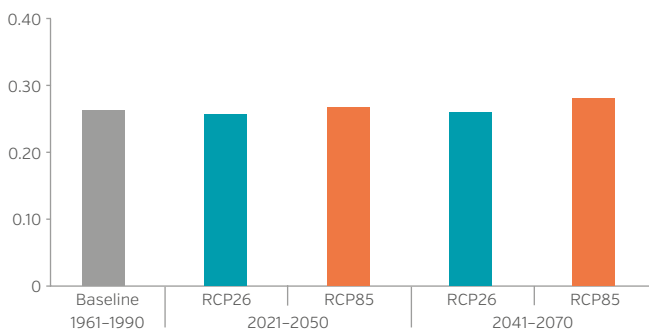
Mean relative vectorial capacity for dengue fever transmission in Jordan
