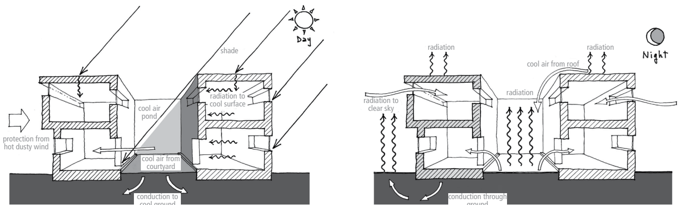
Fig. 04: Cooling system in a courtyard house
