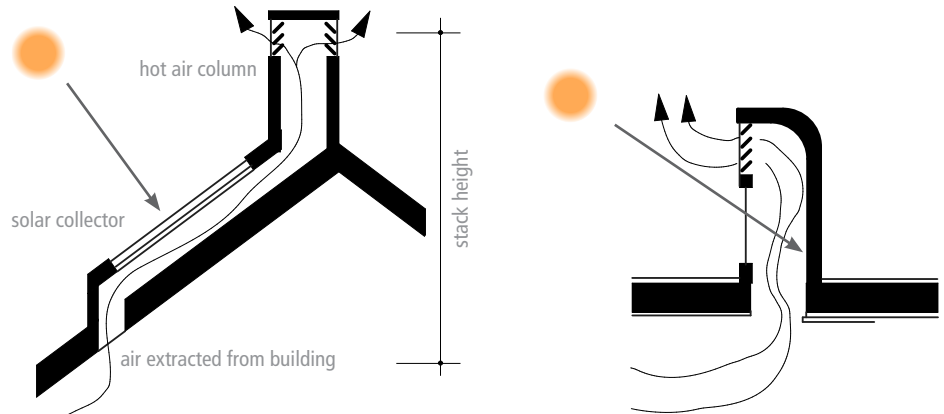
Fig. 05: Examples of solar chimneys
