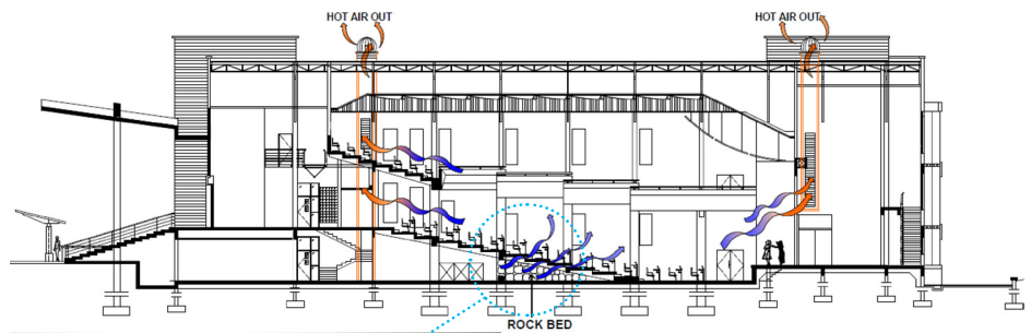
Fig. 07: Rock bed heat exchanger
