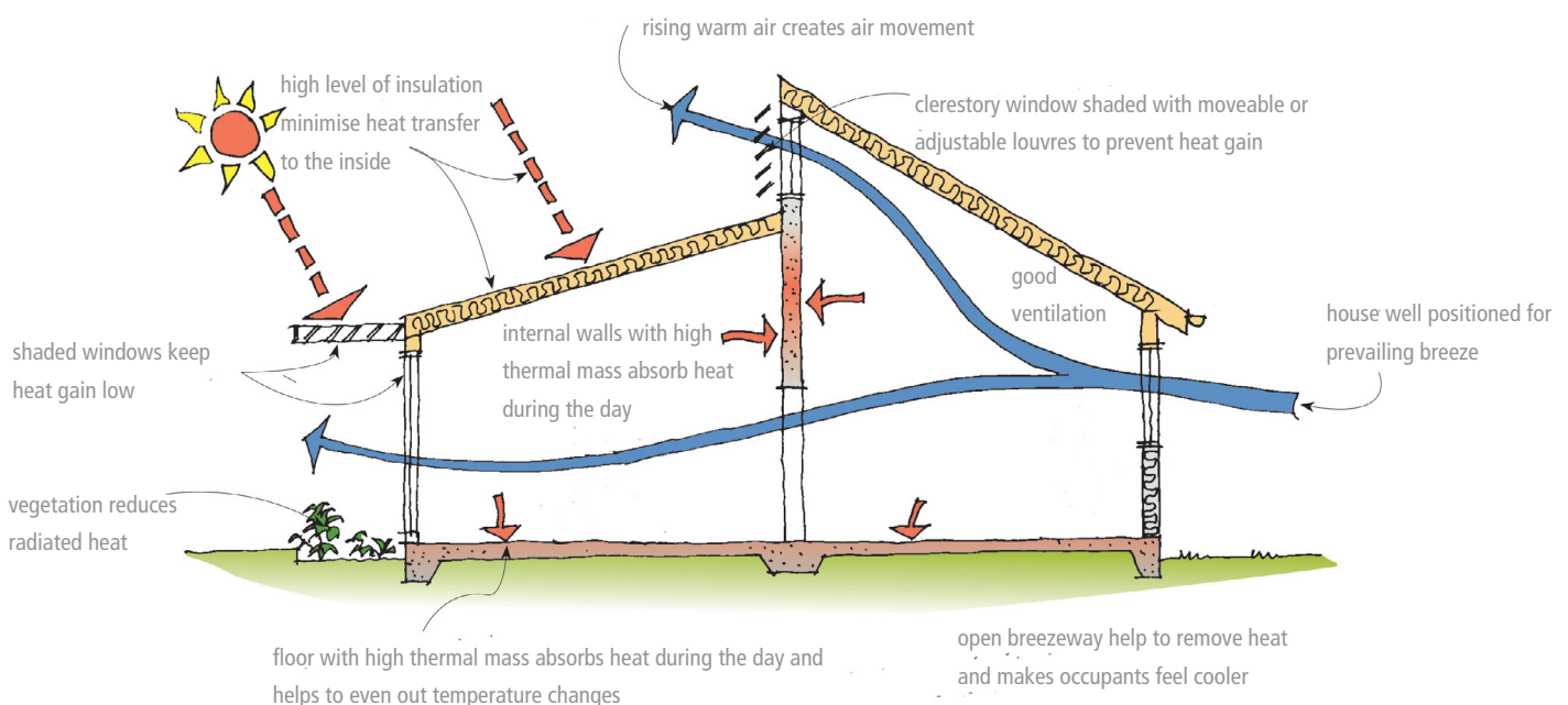
Fig. 01: Features of passive design for cooling
