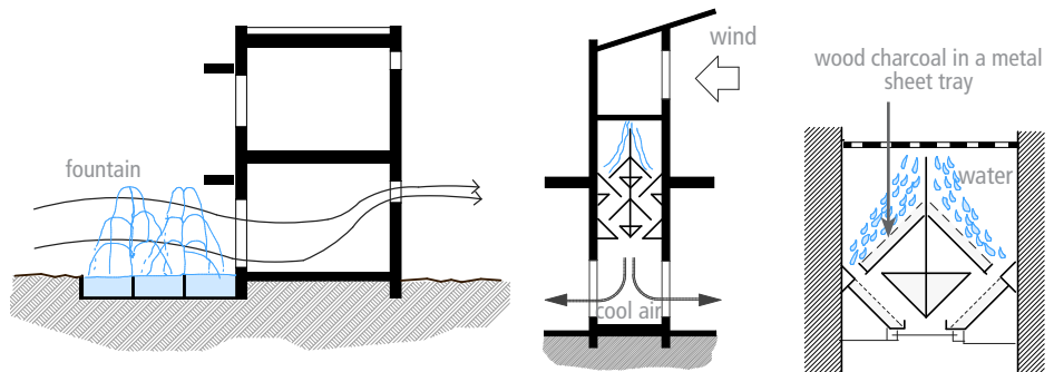
Fig. 03: Evaporative cooling strategies
